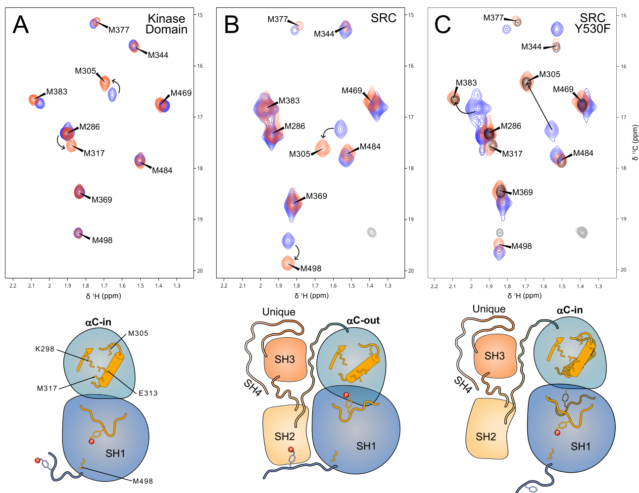
Figure 2. Met-CH 3 ^1\text{H} - ^{13}\text{C} HMQC correlation spectra of unphosphorylated (blue) and phosphorylated (red) Src KD (A), full-length Src (B), and Y530F mutant of full-length Src (C). M317 is on the same face of the C-helix as E313 that forms an essential salt bridge with K298 in the \alpha\text{C-in} conformation and is absent in the \alpha\text{C-out} state. M305 is sensing the activation state of Src. The \alpha\text{C-out} conformation is observed when Y530 is phosphorylated, independent of the phosphorylation state of Y419. When the phosphorylation of Y530 is prevented in the Y530F mutant, phosphorylation of Y419 causes a transition from \alpha\text{C-out} to \alpha\text{C-in} . NMR conditions are the same as in Figure 1.
