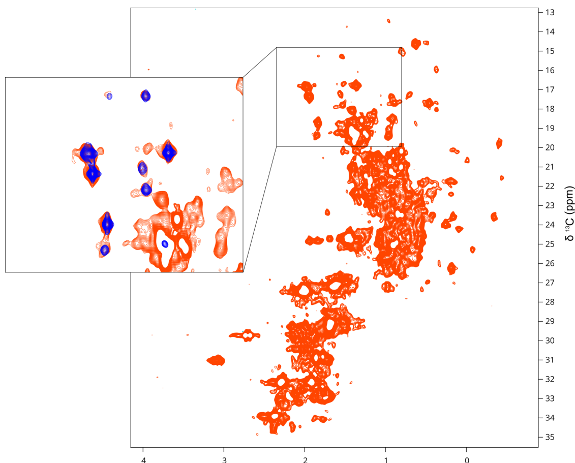
Figure 5. ^1\text{H} – ^{13}\text{C} XL-ALSOFAST HMQC spectrum of a 550\ \mu\text{M} sample of full-length Src obtained at 298 K in a 1 GHz instrument. The expansion shows the Met- \text{CH}_3 region superimposed with a spectrum from a Met- ^{13}\text{CH}_3 enriched sample (blue).
