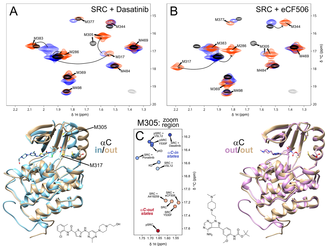
Figure 4. Met-CH 3 ^1\text{H} – ^{13}\text{C} HMQC correlation spectra of unphosphorylated full-length Src in the absence (blue) and in the presence (red) of dasatininb (A) and eCF506 (B) compared to that of the free KD (black). Natural abundance signals from Src are shown in light gray. The models below show the KDs of the autoinhibited form of Src (PDB 2SRC, brown), the eCF506 complex (PDB 7NG7, pink), and the dasatininb complex (PDB 3G5D, blue). (C) Schematic representation of the M305 peak in the different systems studied in this work. The label's colors are assigned automatically in a blue to red scale according to the ^{13}\text{C} chemical shift. The label's colors are assigned automatically in a blue to red scale according to the ^{13}\text{C} chemical shift. NMR conditions are the same as in Figure 1.
