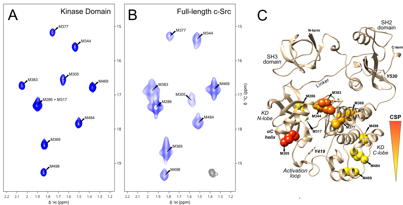
Figure 1. ^1\text{H} – ^{13}\text{C} HMQC correlation spectra of Met- ^{13}\text{CH}_3 -enriched Src KD (A) and full-length Src (B). A natural abundance signal from a nonmethionine methyl group is shown in gray contours. (C) The position of methionine groups is represented on the AlphaFold2 model of full-length Src with colors indicating the combined chemical shift perturbations (CSP) of Met- \text{CH}_3 groups between the full-length protein and the isolated domain. CSP have been calculated as \text{CSP} = (0.5 (\delta_{\text{H}})^2 + (0.185\delta_{\text{C}})^2)^{0.5} based on the average variances of proton and carbon in the BioMagResBank. 19 The protein concentration was ca. 100 \mu\text{M} in 20 mM sodium phosphate, pH = 7.5, 100 mM NaCl, and 0.01% \text{NaN}_3 measured at 298 K in 3 mm tubes. KD and full-length spectra were measured at 600 and 800 MHz, respectively. Additional details are included in materials and experimental methods.
