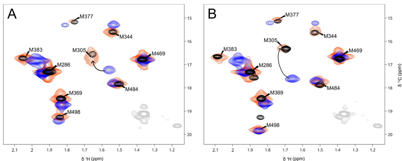
Figure 3. Met-CH 3 ^1\text{H} – ^{13}\text{C} HMQC correlation spectra of unphosphorylated (A) and phosphorylated (B) free Src (blue), VSL12 complex (red), and isolated KD (black). Natural abundance signals from Src and VSL12 peptide are shown in light gray. NMR conditions are the same as in Figure 1.
